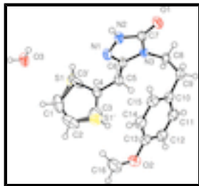
Fig. 1. The molecular structure of the title compound, showing the crystallographic numbering scheme and displacement ellipsoids drawn at the 50% probability level.
